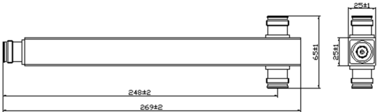
Figure 1 JX-PS-575-6000-2C43DI front panel layout
