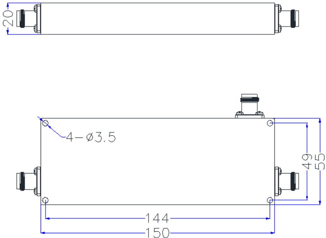
Figure 1 JX-DC-140M500M-Nx front panel layout
