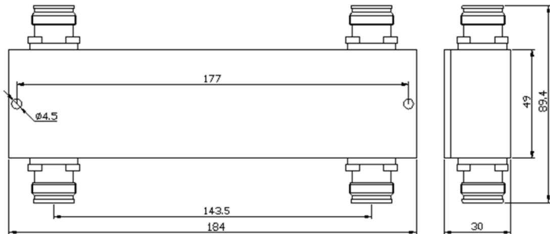
Figure 1 JX-340-2700-3C43DI-B 3dB Hybrid front panel layout
