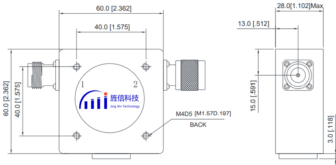
Figure 1 JX-CI-157M159M-60NF front panel layout
