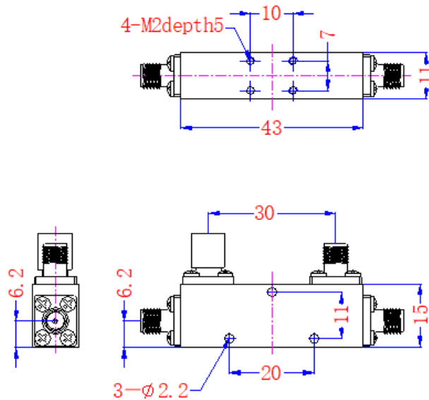
Figure 1 JX-DC-2G8G-30SF front panel layout
