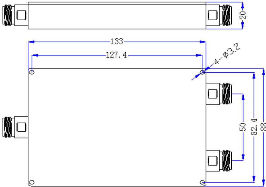
Figure 1 JX-PD-340M2000M-20N front panel layout
