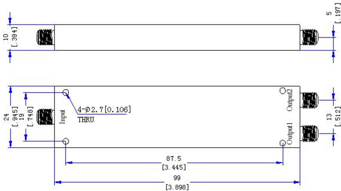
Figure 1 JX-PD2-1G18G-18S front panel layout
