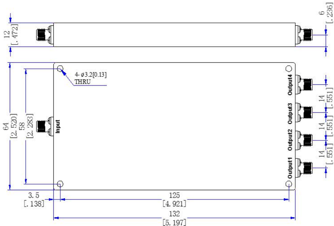
Figure 1 JX-PD4-500M8000M-20S front panel layout
