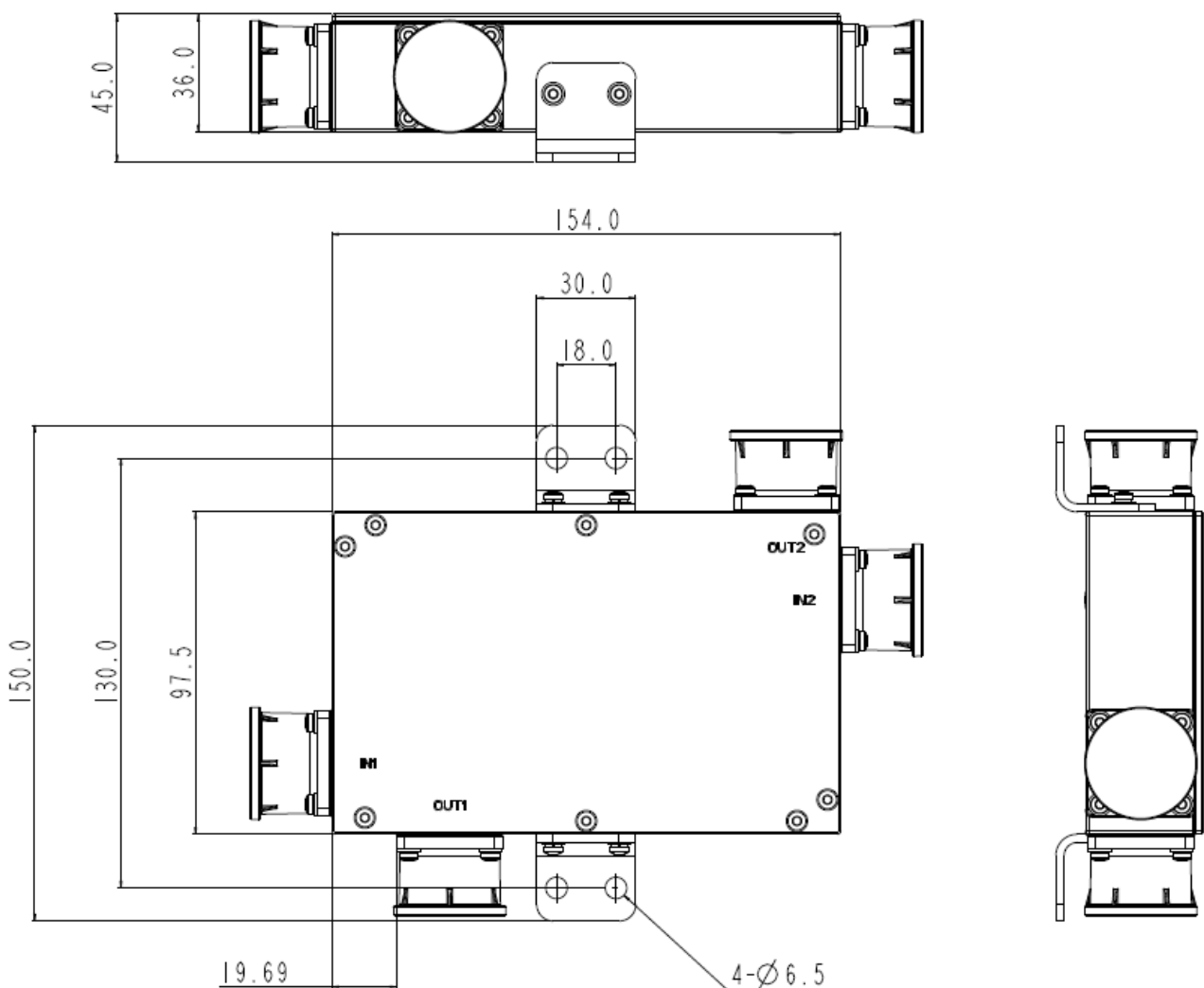
Figure 1 JX-PC-70M500M-20D front panel layout
