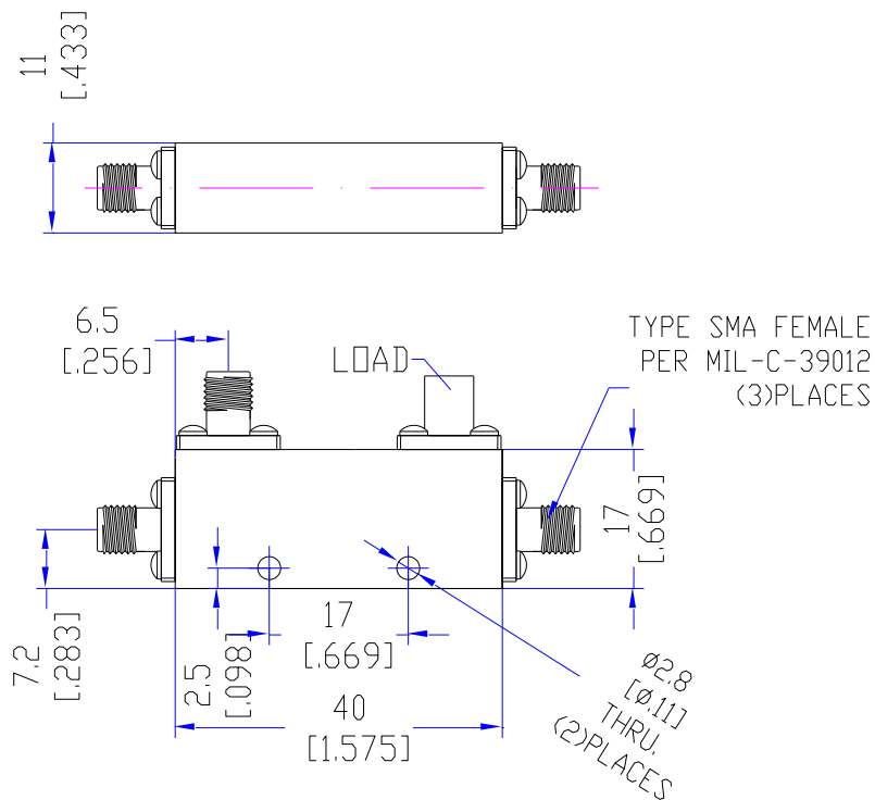
Figure 1 JX-DC-2G18G-6SY front panel layout
