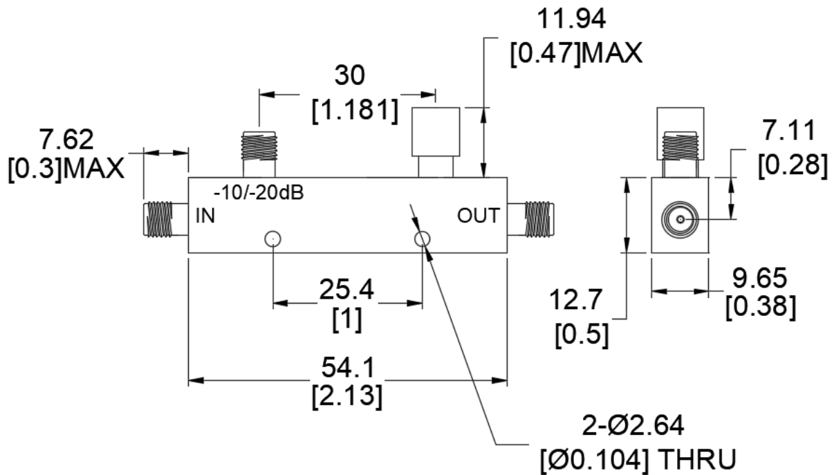
Figure 2 JX-DC-2G18G-10/20SY front panel layout
